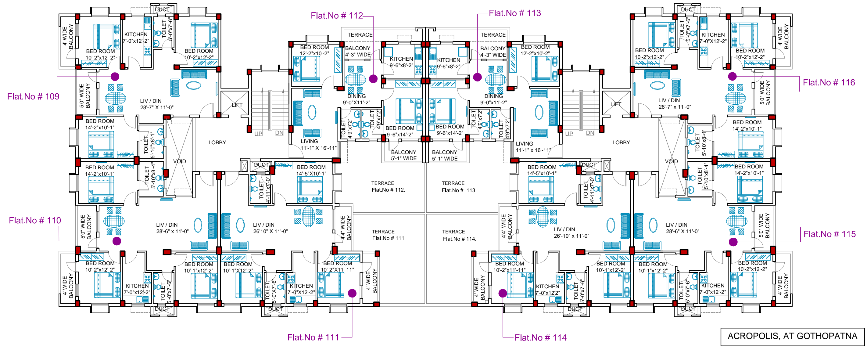
FIRST FLOOR PLAN FOR BLOCK - A
