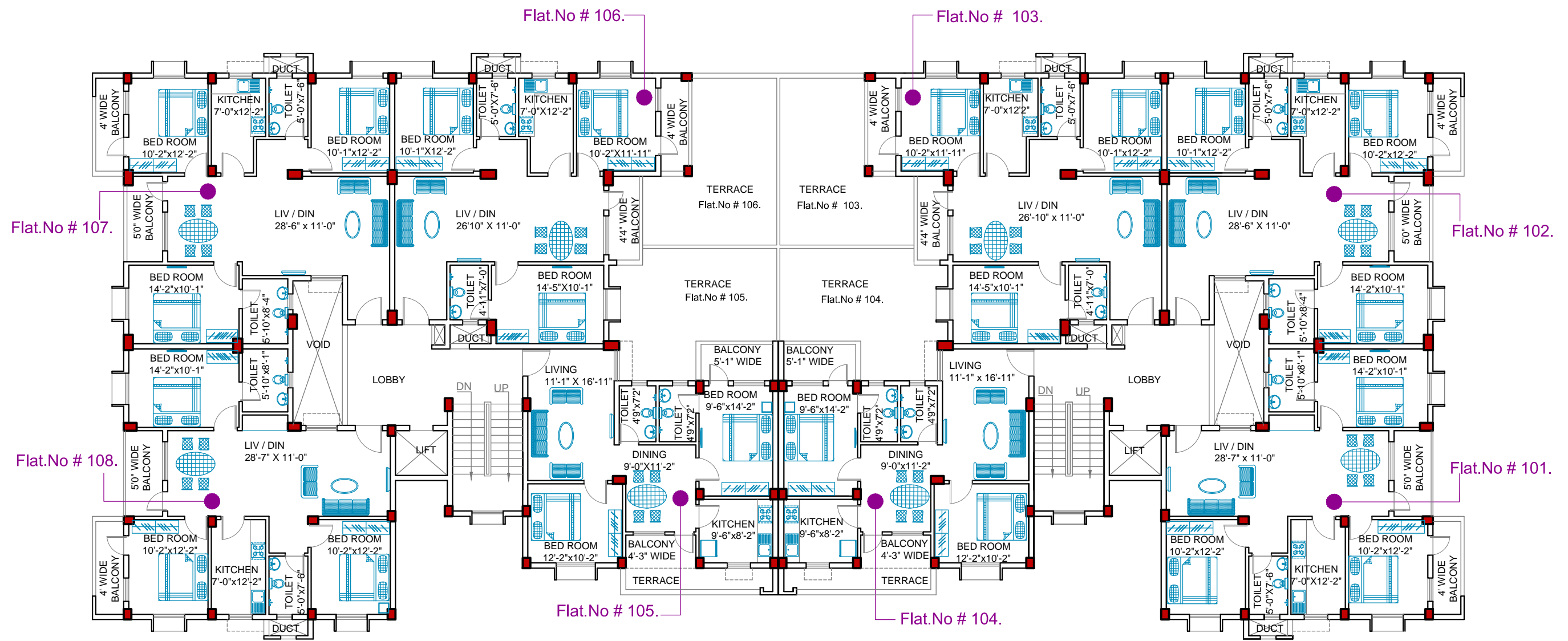
FIRST FLOOR PLAN FOR BLOCK - A
